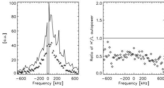
Figure 4: Left: Autopower spectra just before and after the second L-H* transition for volume 1, right: Ratio of H*/L autopower
